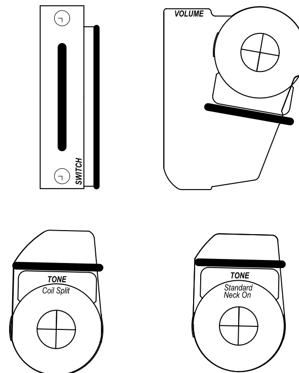
Cut-Out Template
