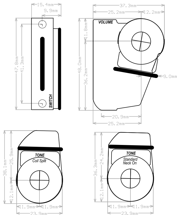
Technical Drawing
